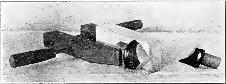
FIG. 570. COPING A MEMBER OF TEE-PIPE PATTERN.
